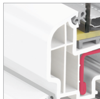
Rounded sash design
