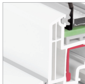
Recessed sash design
