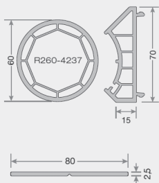
TUBE CONNECTOR (ARTICLE 57061 + R260-4237 / 2 X 57062 / 68068)
