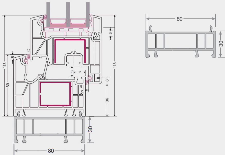
EXTENSION 1,18 IN (ARTICLE 68055)
