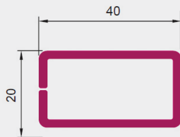
REINFORCEMENT FIXED MULLION 92 (ARTICLE B4020)
