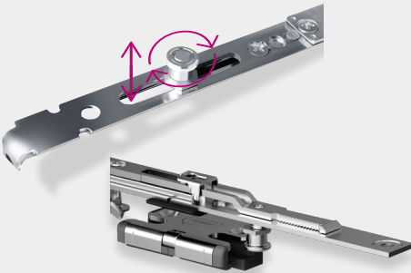
KOPIBO ROLLERS AND ROLLER GUIDE
