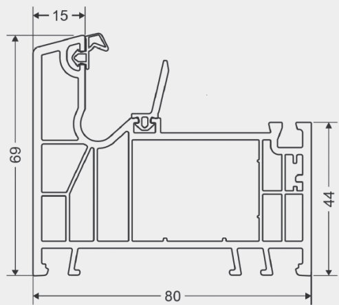
FRAME 69 (ARTICLE 68011 MD)
