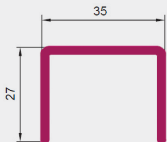
REINFORCEMENT SASH 57 (ARTICLE A3527)
