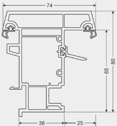
MOVABLE MULLION (ARTICLE 68033)
