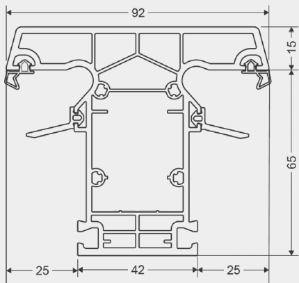
FIXED MULLION 92 (ARTICLE 68032 MD)
