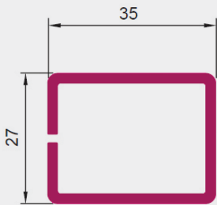
REINFORCEMENT (CLOSED) FRAME 69 (ARTICLE 150B3527)
